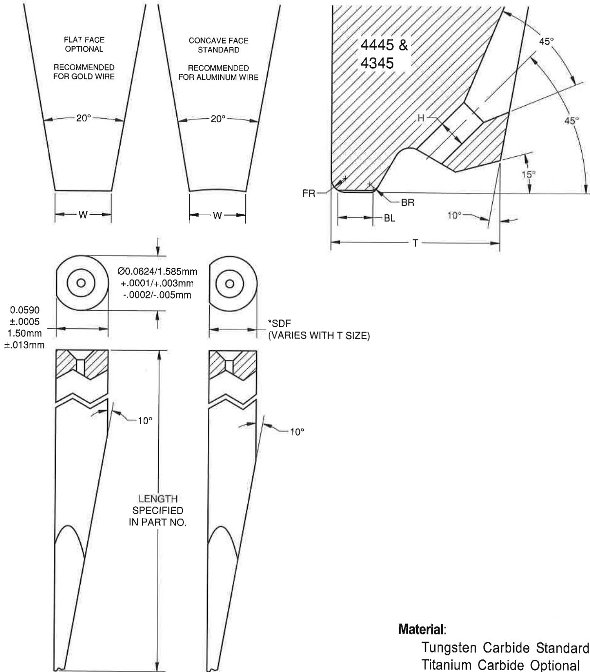
4445 Standard Shank Design
